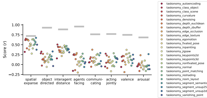
Figure 11: The performance of the taskonomy (Sax et al., 2020; Zamir et al., 2018) models in predicting behavioral responses. Plotting conventions are the same as Figure 2.
