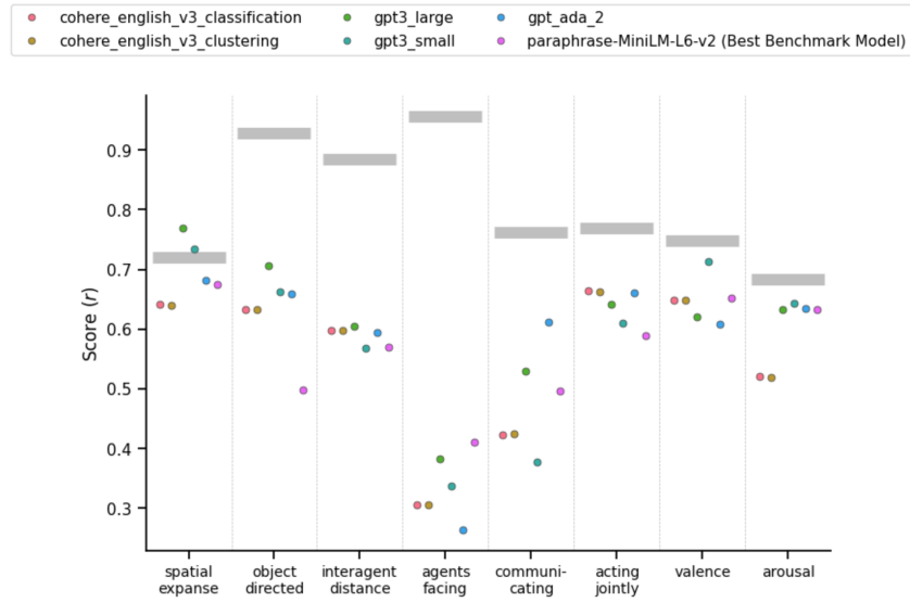
Figure 12: The performance of the GPT-3, GPT Ada-002, and Cohere models compared to the overall best performing model across behavioral ratings. Plotting conventions are the same as Figure 2.
