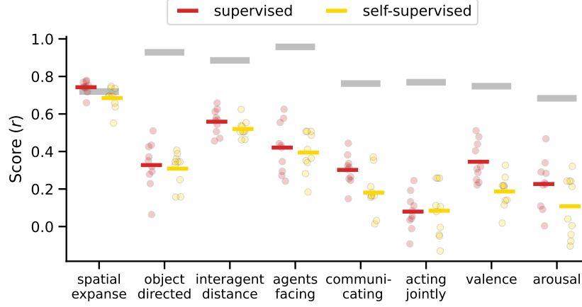
Figure 8: The performance of each image model in our set with a ResNet-50 backbone in predicting behavioral responses separated by whether the model uses a supervised (red) or self-supervised (yellow) learning objective. This analysis was restricted to a single architecture class (ResNet-50) to focus specifically on the learning objective. Plotting conventions are the same as Figure 2.
