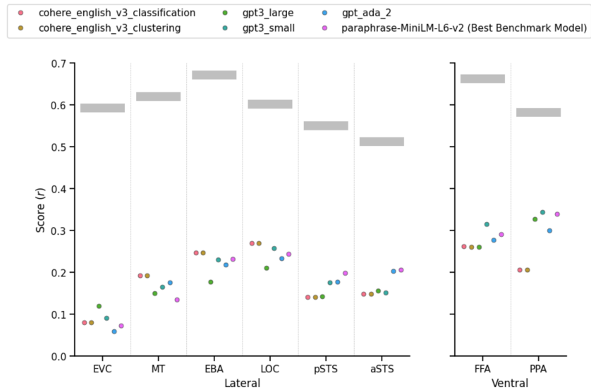
Figure 22: The performance of the GPT-3, GPT Ada-002, and Cohere models compared to the overall best performing model. Plotting conventions are the same as Figure 4.
