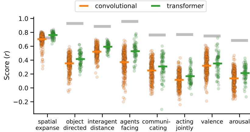
Figure 7: The performance of each image model in our set in predicting behavioral responses separated by whether the model has a convolutional (orange) or transformer (green) architecture. Plotting conventions are the same as Figure 2.
