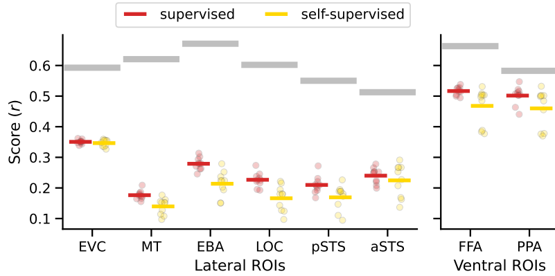
Figure 17: The performance by each image models with a ResNet-50 backbone in predicting neural responses in ROIs in the lateral and ventral visual streams. Models are grouped by supervised (red) or self-supervised (yellow) learning objective. This analysis was restricted to a single architecture class (ResNet-50) to focus specifically on the training objective. Plotting conventions are the same as Figure 4.
