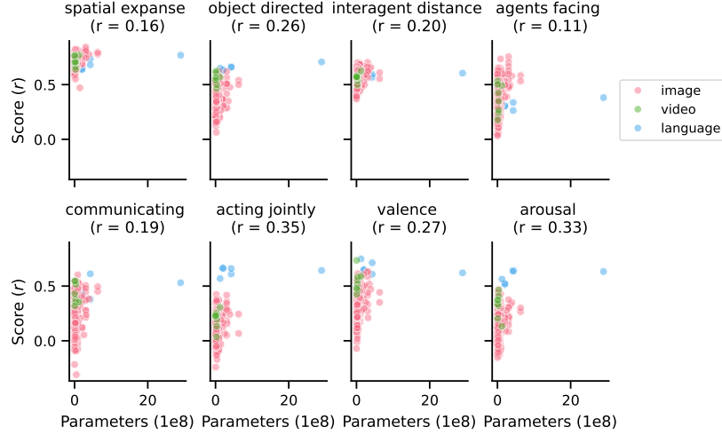
Figure 10: For each behavioral response, the model’s prediction score is plotted against the number of trainable parameters. The r -value below the behavioral response indicates the Pearson correlation between the score and number of trainable parameters.
