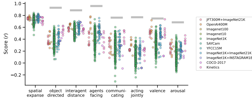
Figure 9: The performance of the vision models (image and video) at predicting the behavioral responses grouped according to their training data. Plotting conventions are the same as Figure 2.
