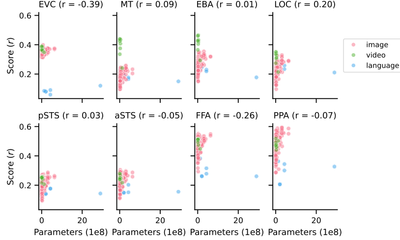
Figure 20: For each ROI response, the model’s prediction score is plotted against the number of trainable parameters. The r-value next to the ROI response indicates the Pearson correlation between the score and number of trainable parameters.
